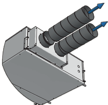
Plenum standard DEH 2: 2 attacchi Ø 160 mm (per DEH 1: 1 attacco Ø 160 mm)
