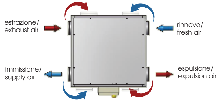
DUO-ED V - VIEW FROM THE TOP Configurazione standard DUO-ED V - VIEW FROM THE TOP Configurazione standard
