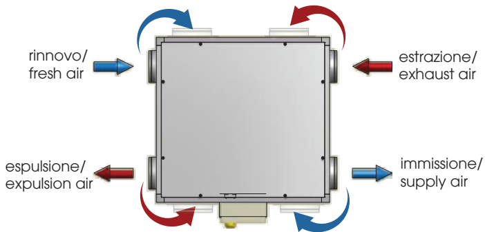
DUO-ED V - VIEW FROM THE TOP Configurazione standard DUO-ED V - VIEW FROM THE TOP Configurazione standard
