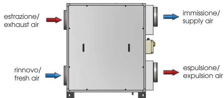
DUO-ED V - VIEW FROM THE TOP Configurazione standard DUO-ED V - VIEW FROM THE TOP Configurazione standard
