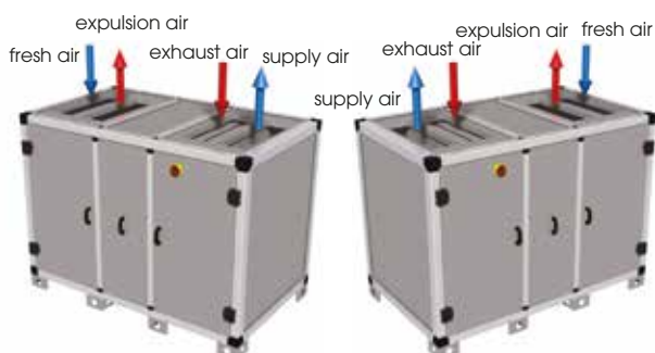
UVR-TOP from size 3 to 6 standard and mirrored configuration
