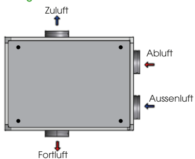
Konfiguration 4 Standard
