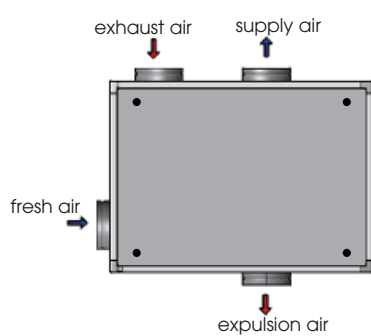
Configuration 3 Mirrored
