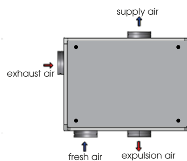
Configuration 2 Mirrored
